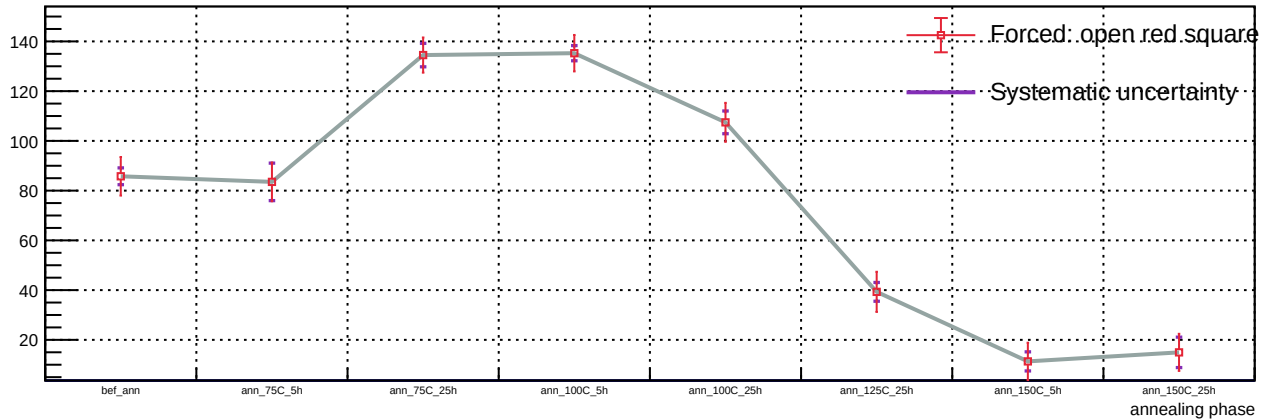
Sensor A1, v = 5 V, representative T = 23 C (max available) - Spot 82: luminosity vs phase
