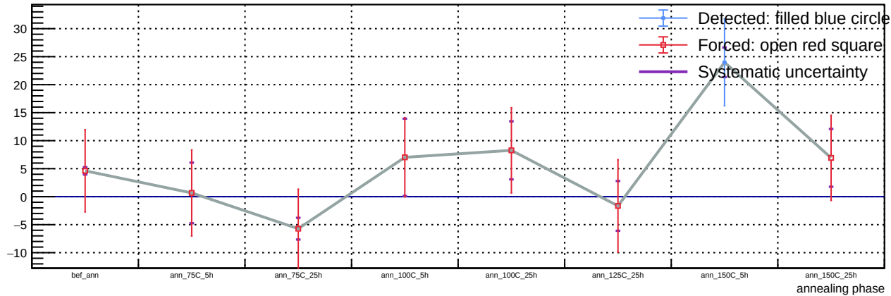
Sensor A1, v = 5 V, representative T = 23 C (max available) - Spot 89: luminosity vs phase
