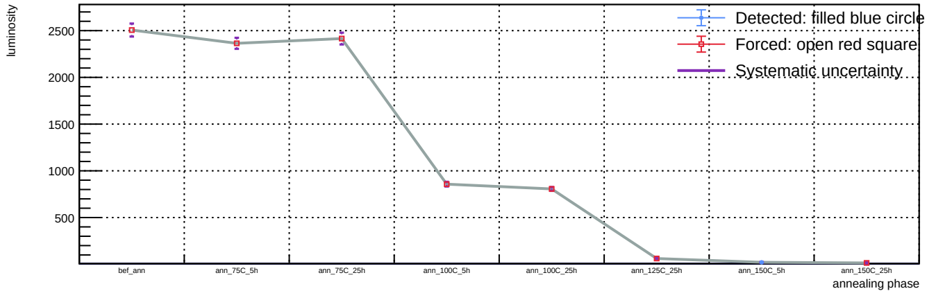
Sensor A1, v = 5 V, representative T = 23 C (max available) - Spot 91: luminosity vs phase
