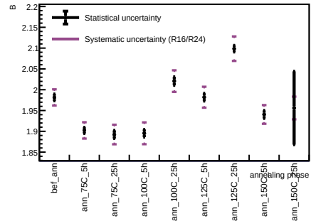
Sensor B1, T = 20 C - Spot 26
