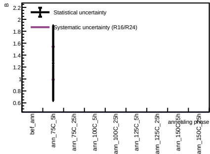
Sensor B1, T = 20 C - Spot 72
