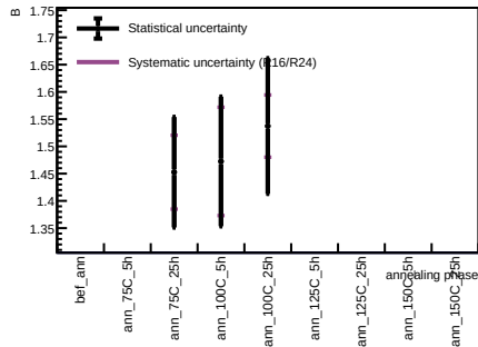
Sensor B1, T = 20 C - Spot 76
