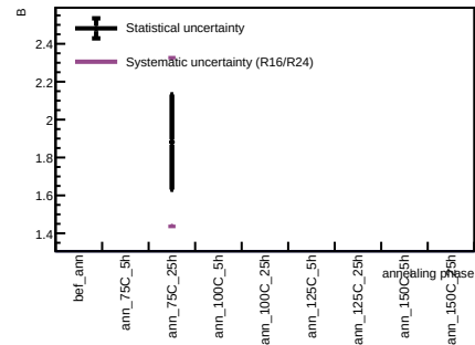
Sensor B1, T = 20 C - Spot 77
