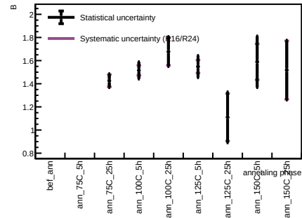
Sensor B1, T = 20 C - Spot 74
