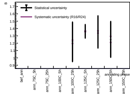
Sensor B1, T = 20 C - Spot 92
