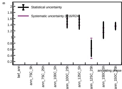
Sensor B1, T = 20 C - Spot 94
