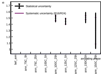
Sensor B1, T = 20 C - Spot 91
