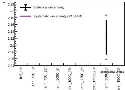
Sensor B1, T = 20 C - Spot 111
