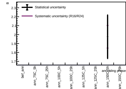
Sensor B1, T = 20 C - Spot 113
