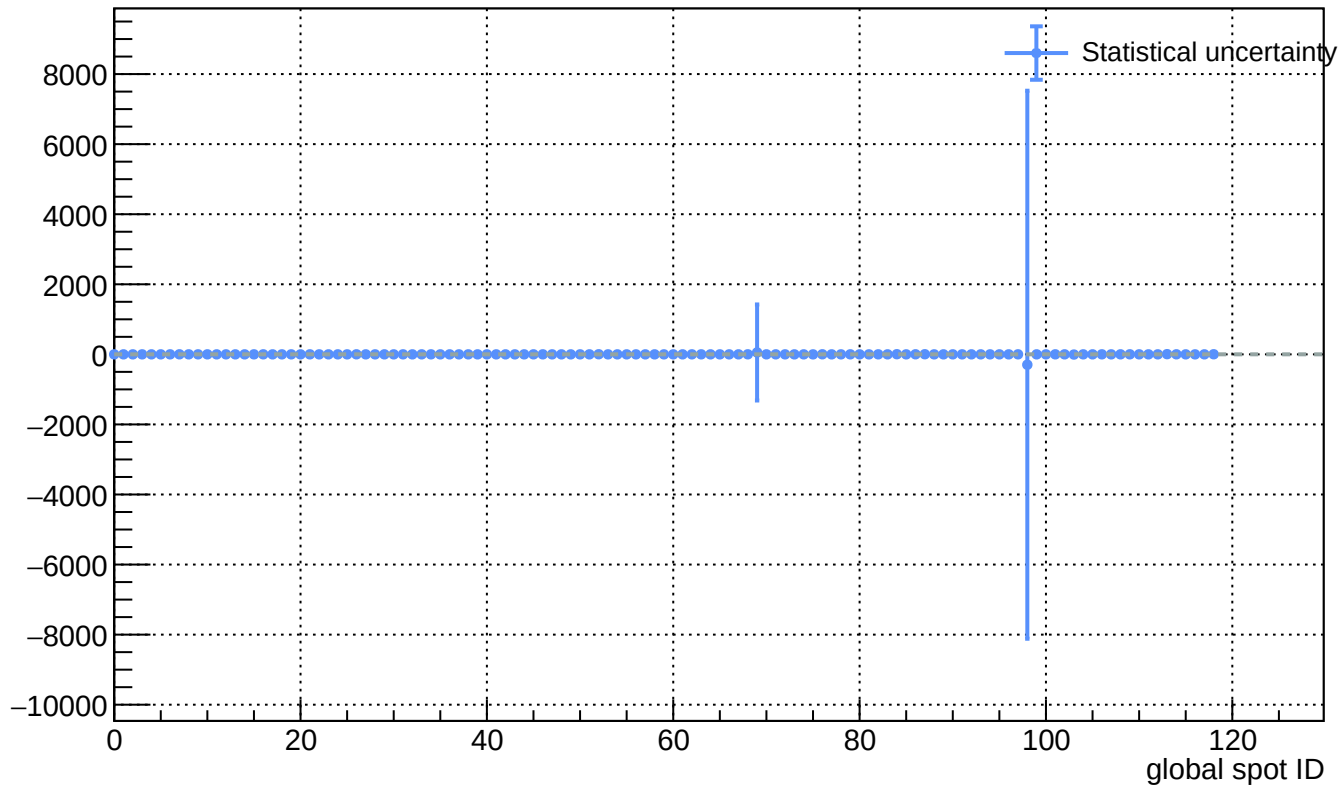
Sensor B1, T = 20 C - L(ann_125C_25h) / L(before_annealing)
