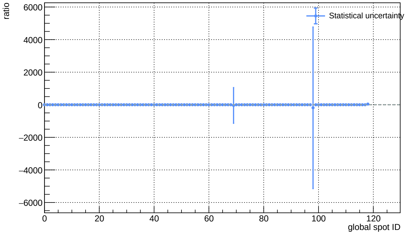
Sensor B1, T = 20 C - L(ann_150C_25h) / L(before_annealing)
