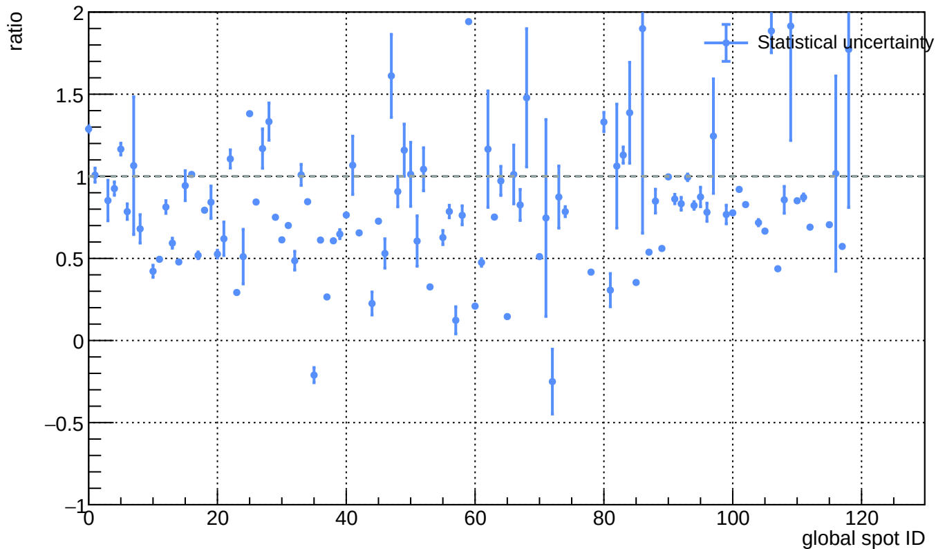
Sensor B1, T = 20\text{ C} - L(\text{ann\_75C\_25h}) / L(\text{before\_annealing})
