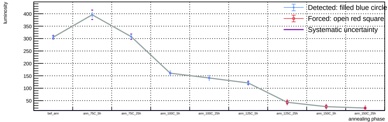
Sensor B1, T = 20 C, representative v = 55.9 V (max available) - Spot 1: luminosity vs phase
