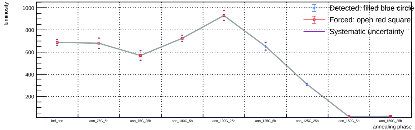
Sensor B1, T = 20 C, representative v = 55.9 V (max available) - Spot 102: luminosity vs phase
