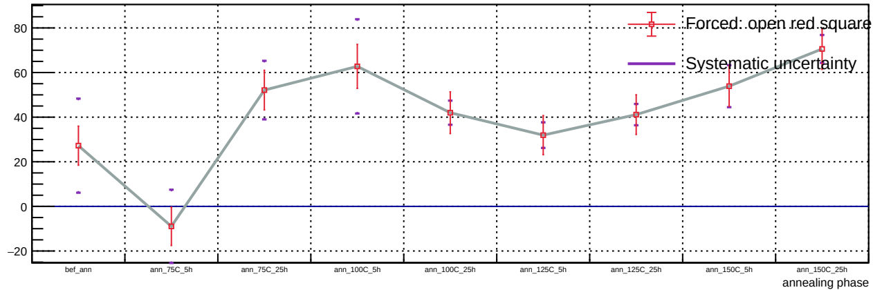
Sensor B1, T = 20 C, representative v = 55.9 V (max available) - Spot 109: luminosity vs phase
