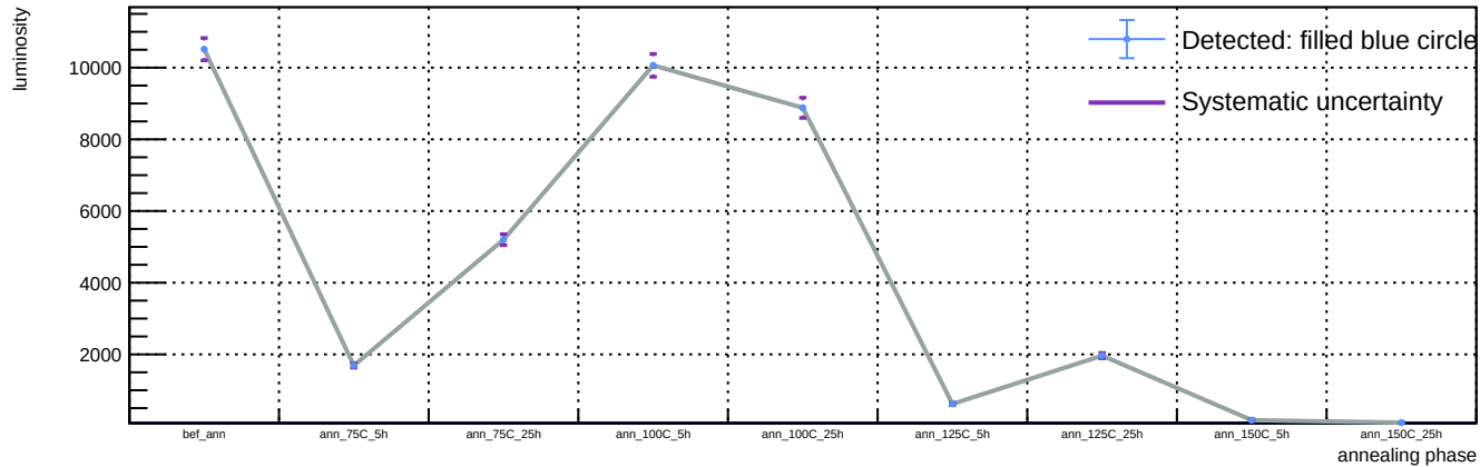
Sensor B1, T = 20 C, representative v = 55.9 V (max available) - Spot 11: luminosity vs phase
