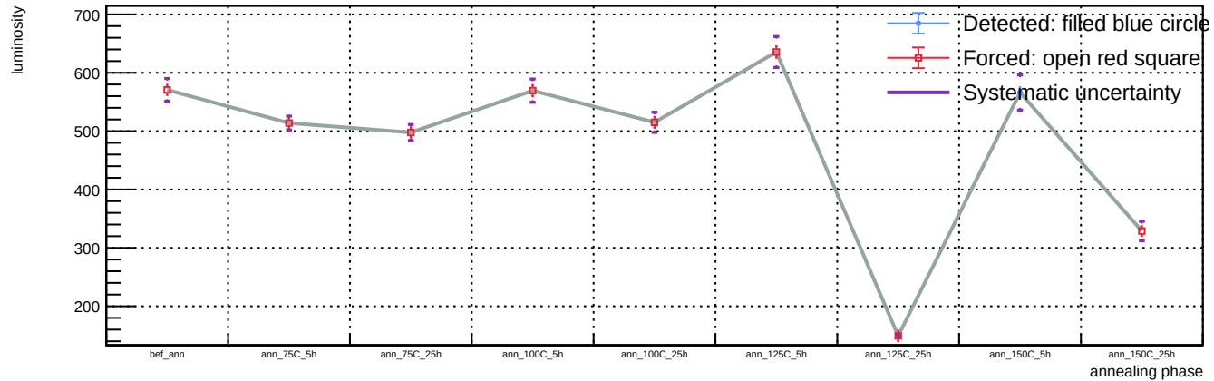
Sensor B1, T = 20 C, representative v = 55.9 V (max available) - Spot 111: luminosity vs phase
