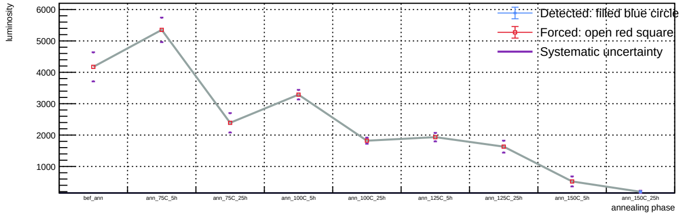
Sensor B1, T = 20 C, representative v = 55.9 V (max available) - Spot 117: luminosity vs phase
