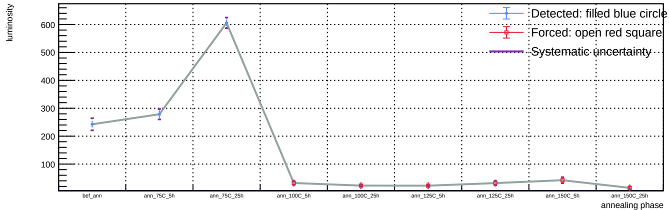
Sensor B1, T = 20 C, representative v = 55.9 V (max available) - Spot 2: luminosity vs phase
