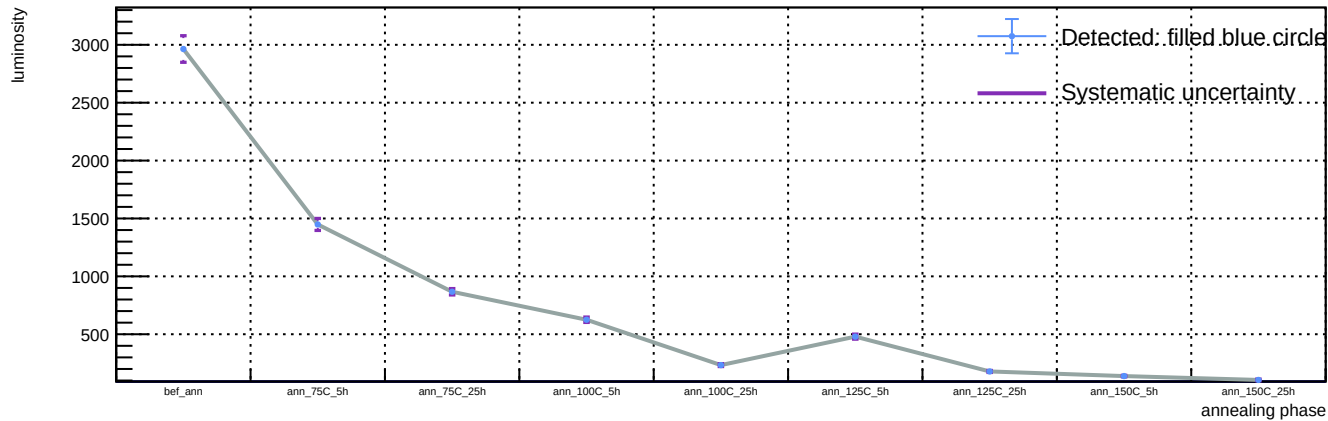
Sensor B1, T = 20 C, representative v = 55.9 V (max available) - Spot 23: luminosity vs phase
