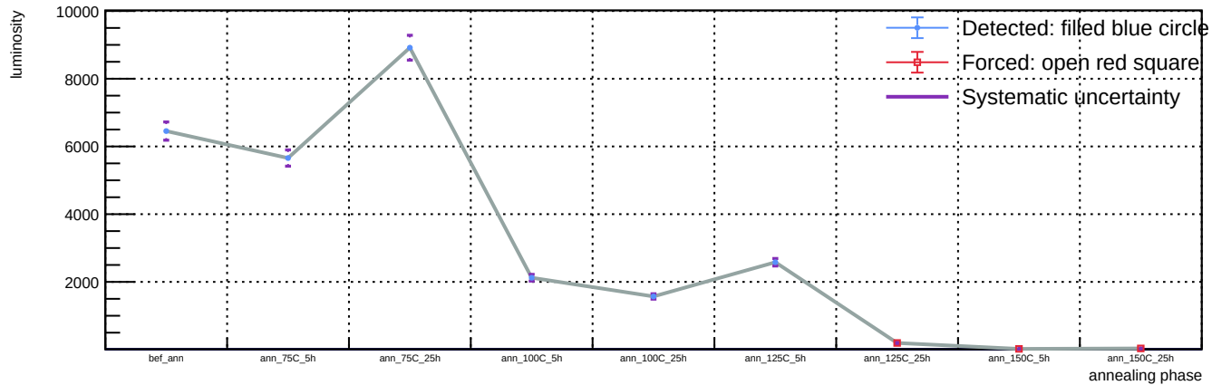
Sensor B1, T = 20 C, representative v = 55.9 V (max available) - Spot 25: luminosity vs phase
