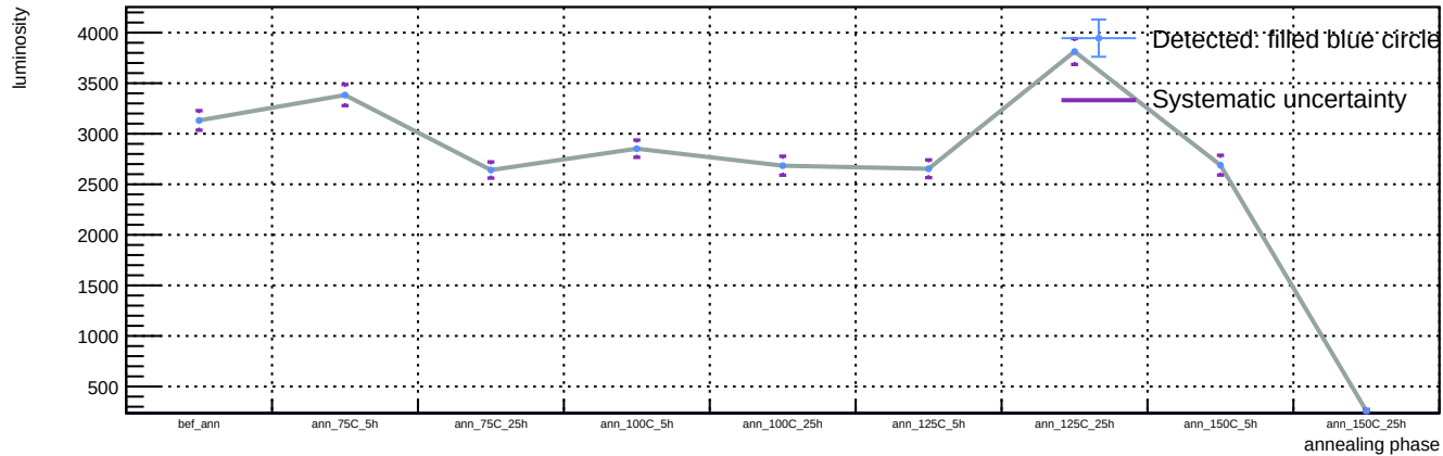
Sensor B1, T = 20 C, representative v = 55.9 V (max available) - Spot 26: luminosity vs phase
