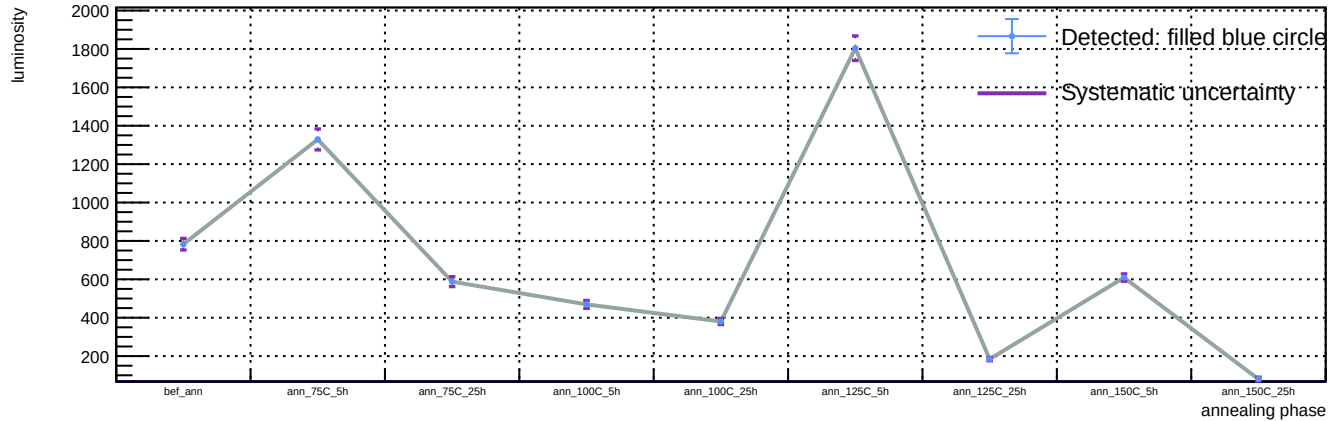
Sensor B1, T = 20 C, representative v = 55.9 V (max available) - Spot 29: luminosity vs phase
