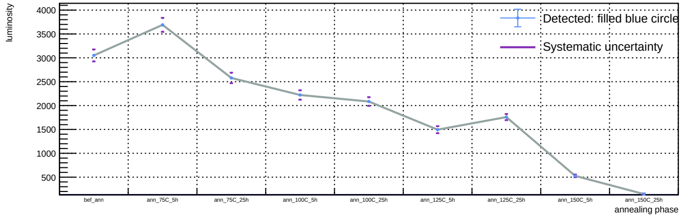
Sensor B1, T = 20 C, representative v = 55.9 V (max available) - Spot 34: luminosity vs phase
