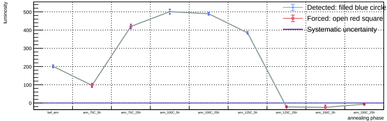
Sensor B1, T = 20 C, representative v = 55.9 V (max available) - Spot 43: luminosity vs phase
