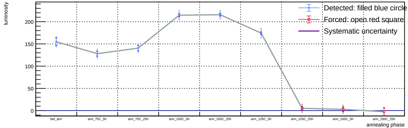
Sensor B1, T = 20 C, representative v = 55.9 V (max available) - Spot 48: luminosity vs phase
