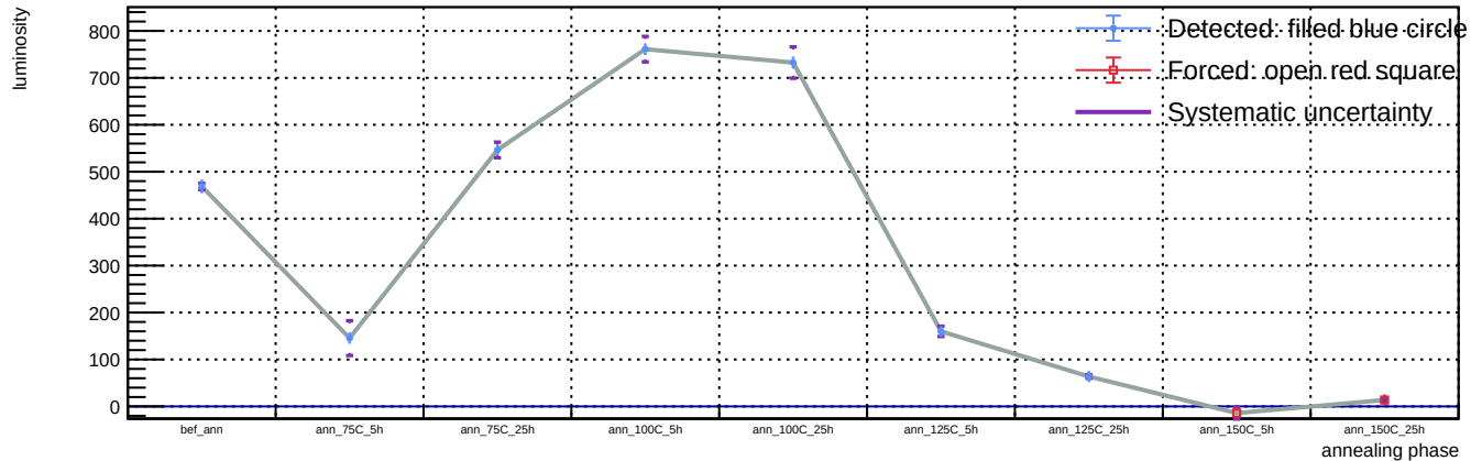
Sensor B1, T = 20 C, representative v = 55.9 V (max available) - Spot 5: luminosity vs phase
