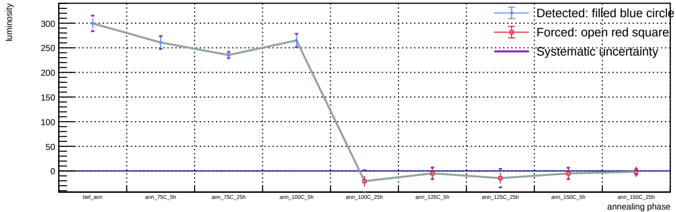
Sensor B1, T = 20 C, representative v = 55.9 V (max available) - Spot 56: luminosity vs phase
