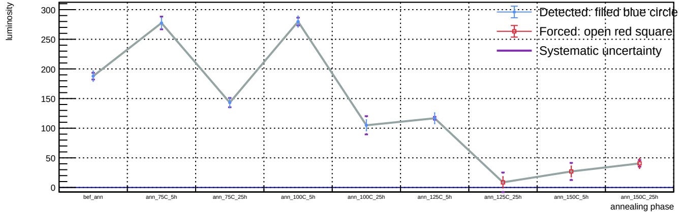
Sensor B1, T = 20 C, representative v = 55.9 V (max available) - Spot 58: luminosity vs phase
