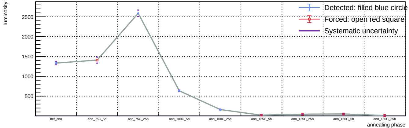
Sensor B1, T = 20 C, representative v = 55.9 V (max available) - Spot 59: luminosity vs phase
