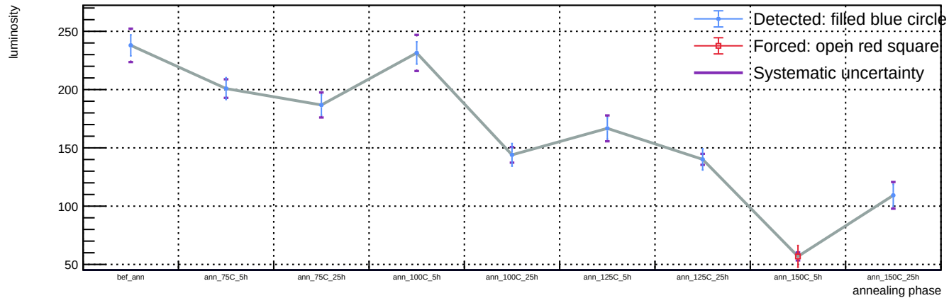
Sensor B1, T = 20 C, representative v = 55.9 V (max available) - Spot 6: luminosity vs phase
