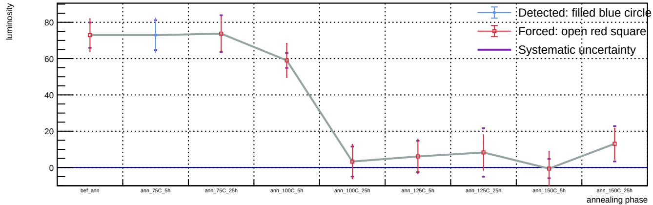
Sensor B1, T = 20 C, representative v = 55.9 V (max available) - Spot 66: luminosity vs phase
