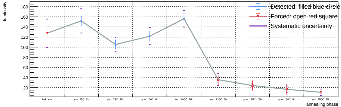
Sensor B1, T = 20 C, representative v = 55.9 V (max available) - Spot 67: luminosity vs phase
