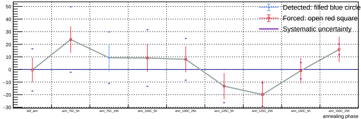
Sensor B1, T = 20 C, representative v = 55.9 V (max available) - Spot 69: luminosity vs phase
