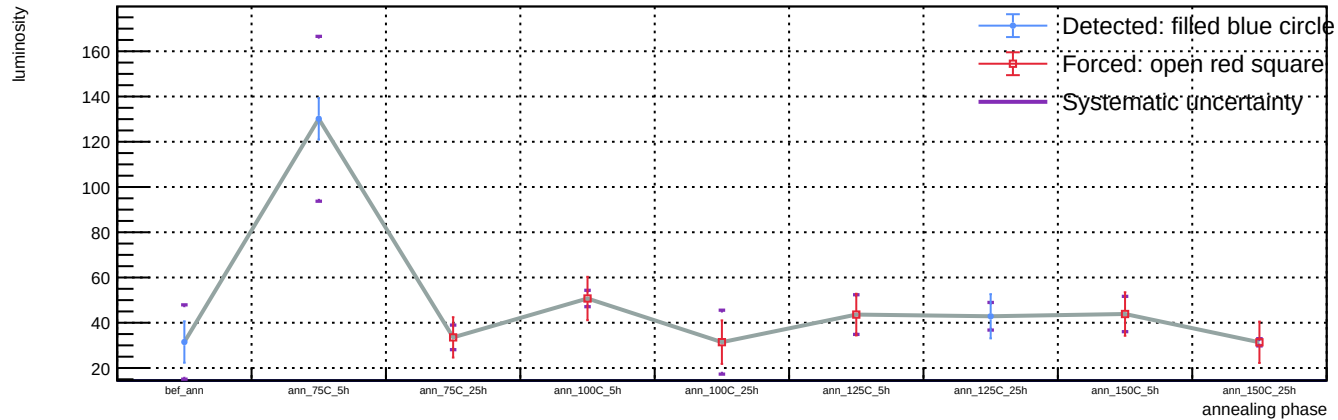
Sensor B1, T = 20 C, representative v = 55.9 V (max available) - Spot 7: luminosity vs phase
