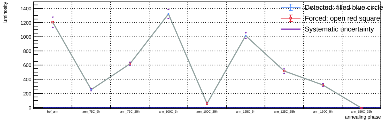
Sensor B1, T = 20 C, representative v = 55.9 V (max available) - Spot 70: luminosity vs phase
