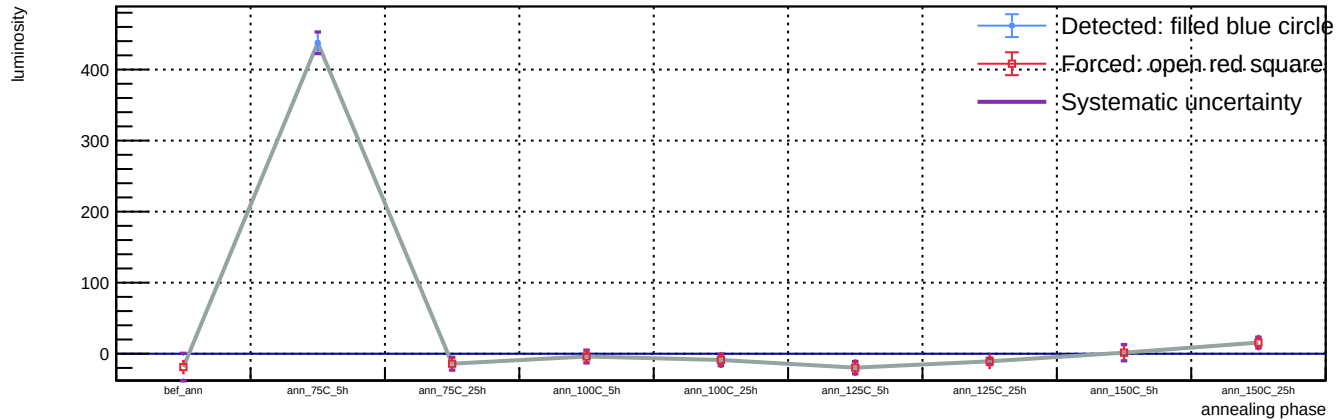
Sensor B1, T = 20 C, representative v = 55.9 V (max available) - Spot 71: luminosity vs phase
