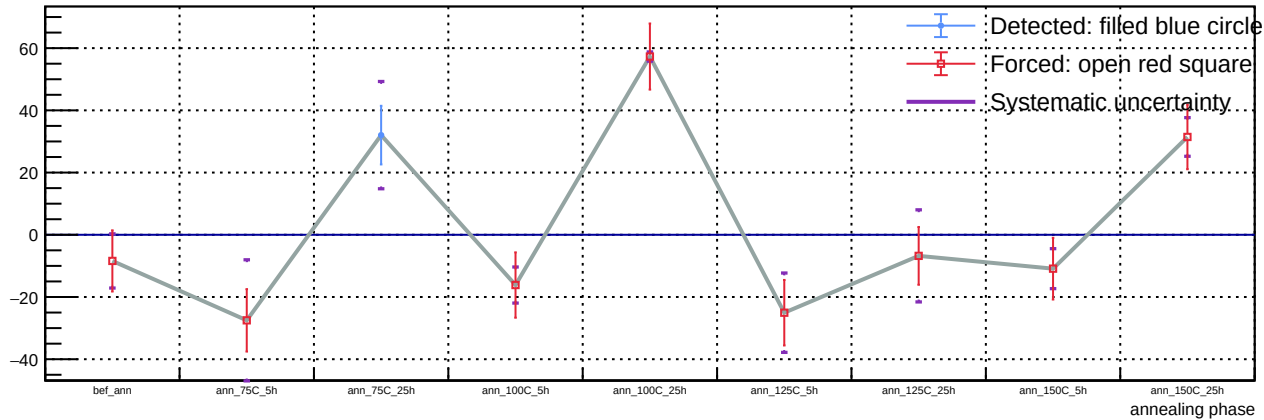
Sensor B1, T = 20 C, representative v = 55.9 V (max available) - Spot 79: luminosity vs phase
