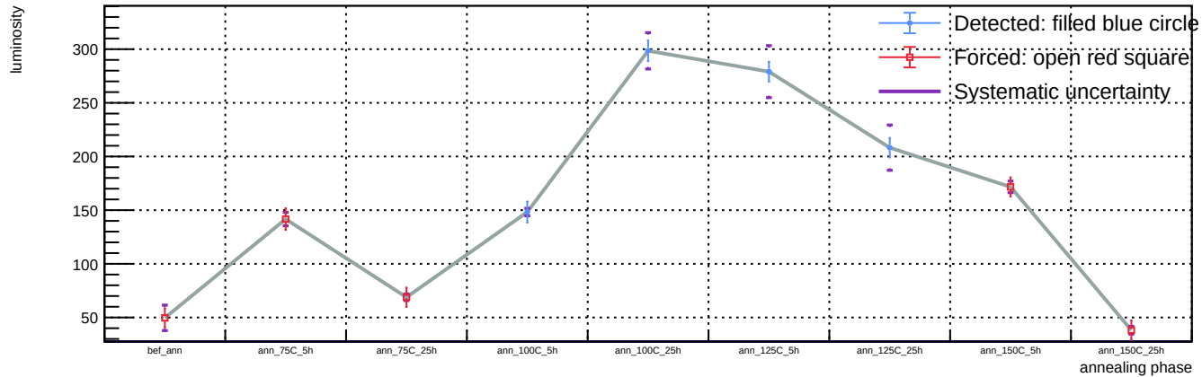
Sensor B1, T = 20 C, representative v = 55.9 V (max available) - Spot 84: luminosity vs phase
