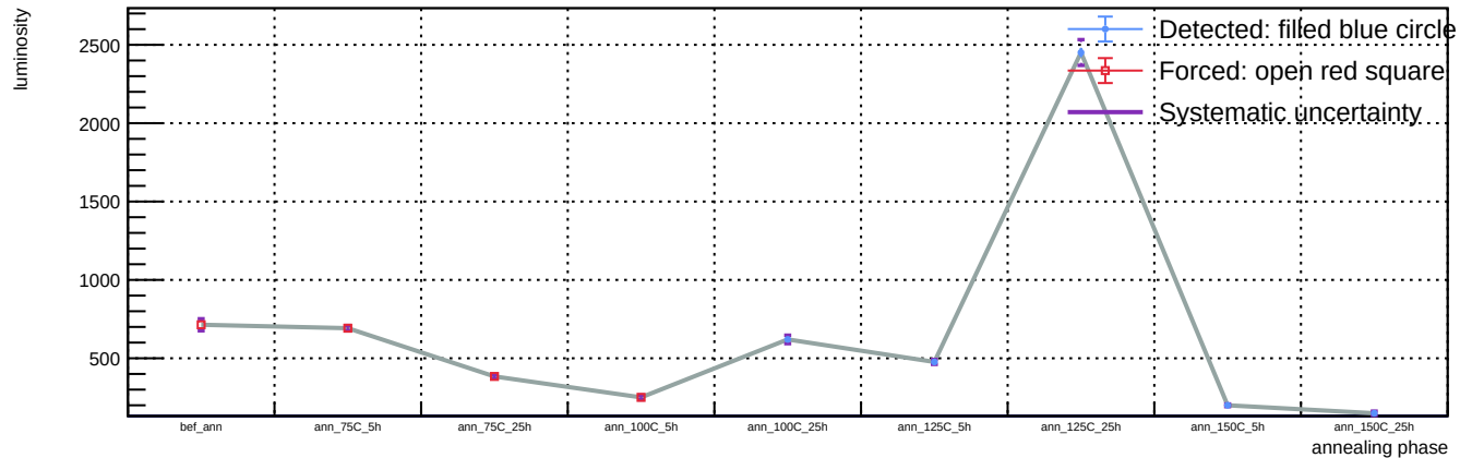
Sensor B1, T = 20 C, representative v = 55.9 V (max available) - Spot 87: luminosity vs phase
