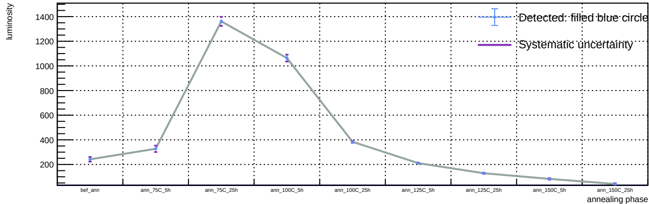
Sensor B1, T = 20 C, representative v = 55.9 V (max available) - Spot 9: luminosity vs phase
