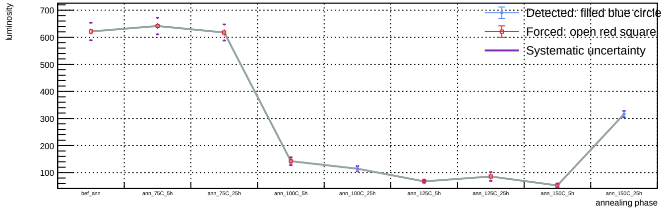
Sensor B1, T = 20 C, representative v = 55.9 V (max available) - Spot 93: luminosity vs phase
