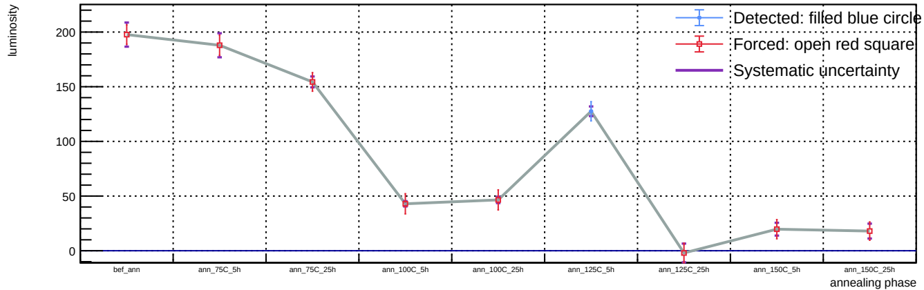
Sensor B1, T = 20 C, representative v = 55.9 V (max available) - Spot 96: luminosity vs phase
