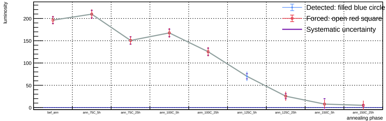
Sensor B1, T = 20 C, representative v = 55.9 V (max available) - Spot 99: luminosity vs phase
