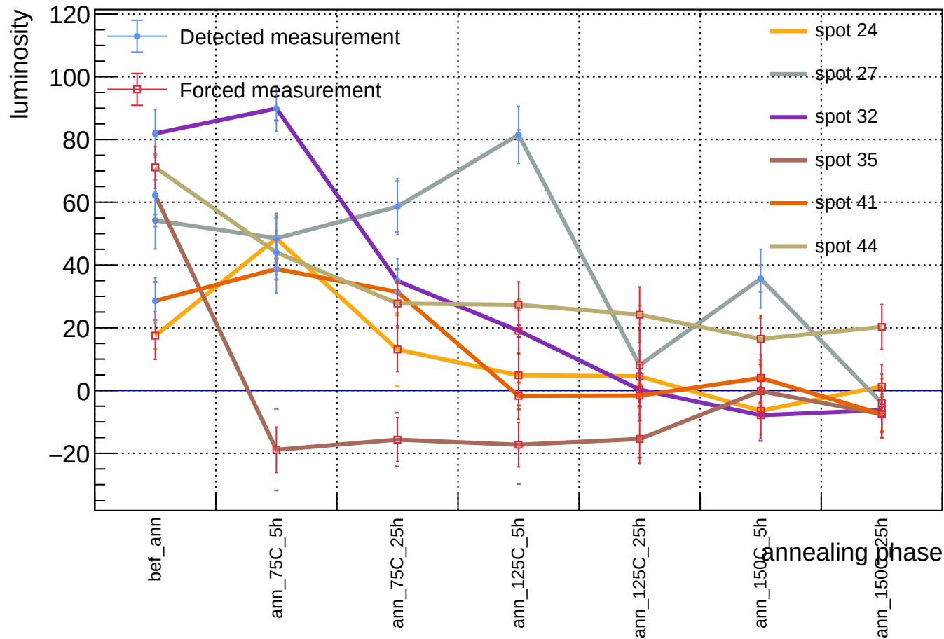
Sensor B1, v = 3 V, representative T = 23 C (max available) - luminosity vs phase - order 10^1
