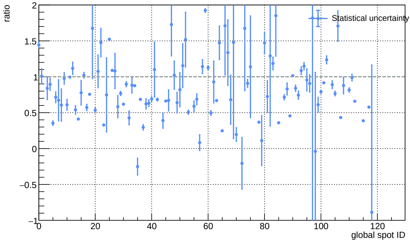
Sensor B1, v = 3\text{ V} - L(\text{ann\_75C\_25h}) / L(\text{before\_annealing})
