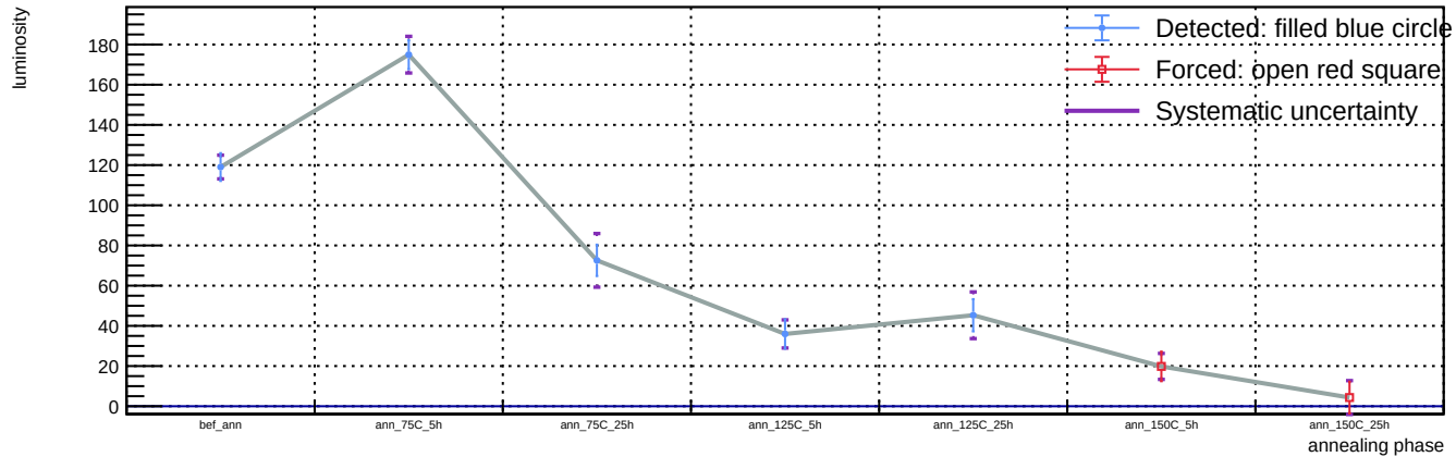
Sensor B1, v = 3 V, representative T = 23 C (max available) - Spot 10: luminosity vs phase
