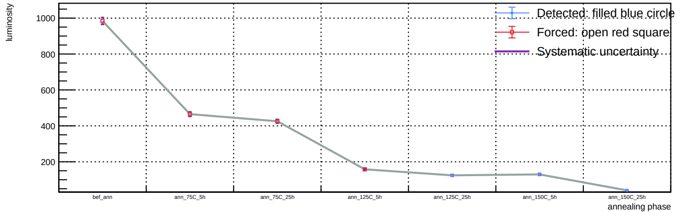
Sensor B1, v = 3 V, representative T = 23 C (max available) - Spot 107: luminosity vs phase
