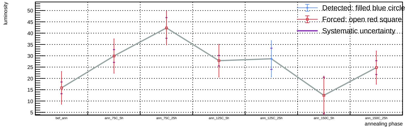
Sensor B1, v = 3 V, representative T = 23 C (max available) - Spot 109: luminosity vs phase
