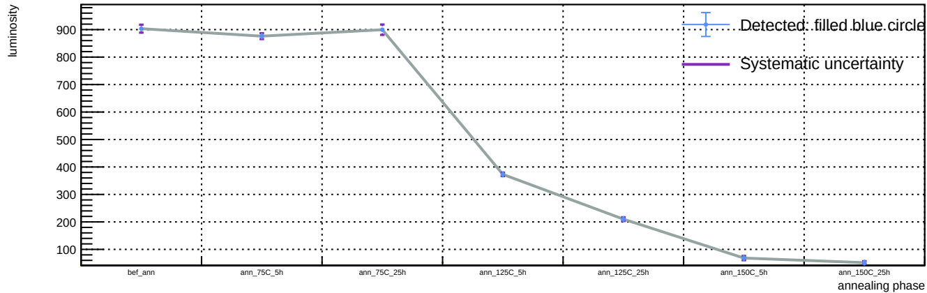
Sensor B1, v = 3 V, representative T = 23 C (max available) - Spot 11: luminosity vs phase
