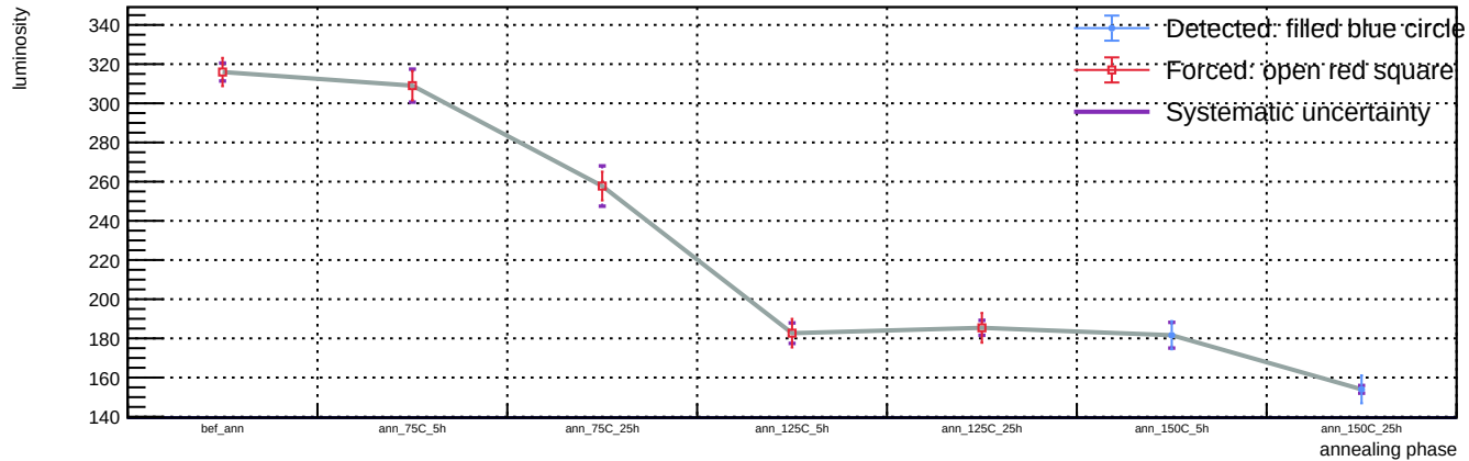
Sensor B1, v = 3 V, representative T = 23 C (max available) - Spot 110: luminosity vs phase
