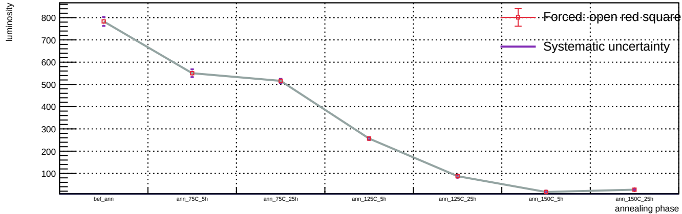
Sensor B1, v = 3 V, representative T = 23 C (max available) - Spot 112: luminosity vs phase
